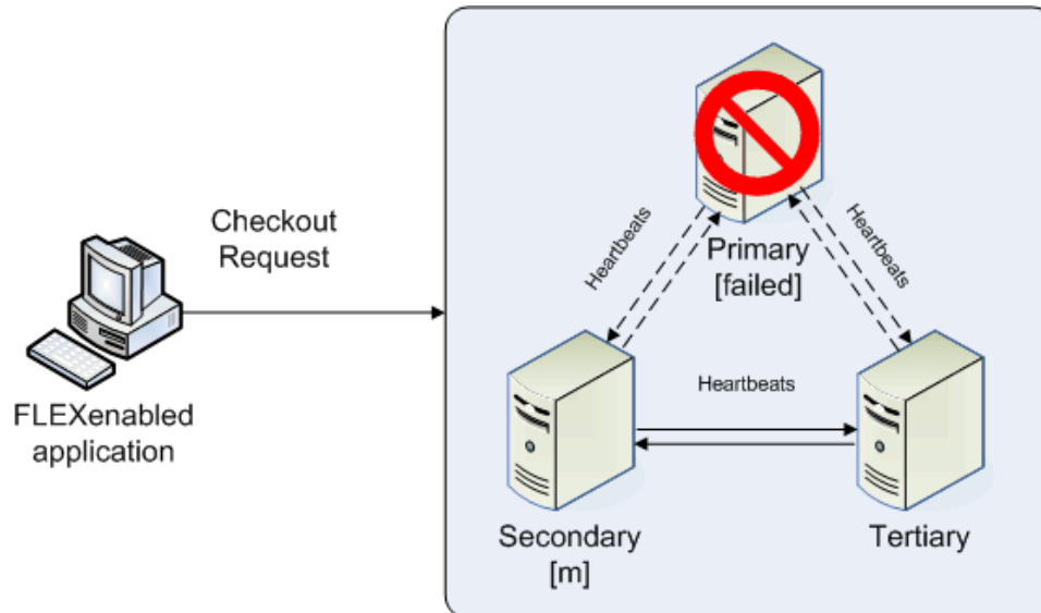
Figure 7-2: Three-Server Redundancy Backup Failover
